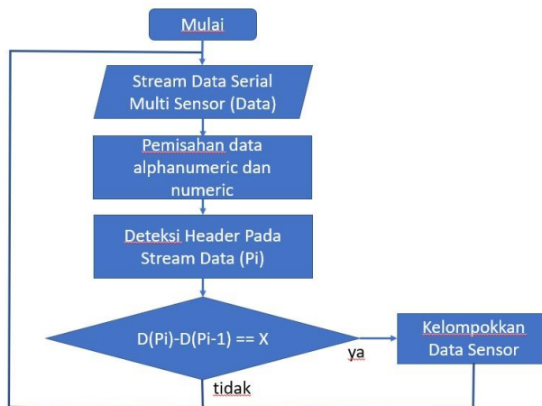
Gambar 3. Filterisasi data raw multi sensor
